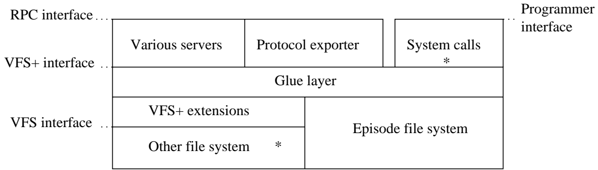
Figure 1: File server organization
